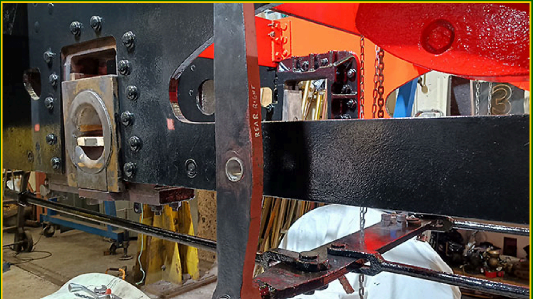
Brake rigging being erected.
